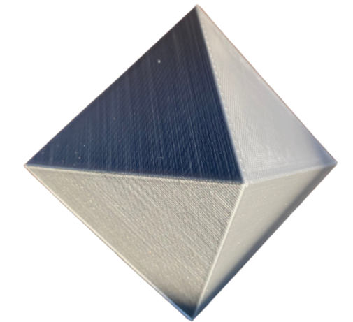
OCTAEDRO
