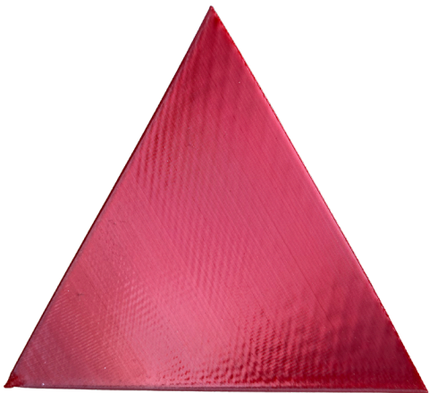
TETRAEDRO
